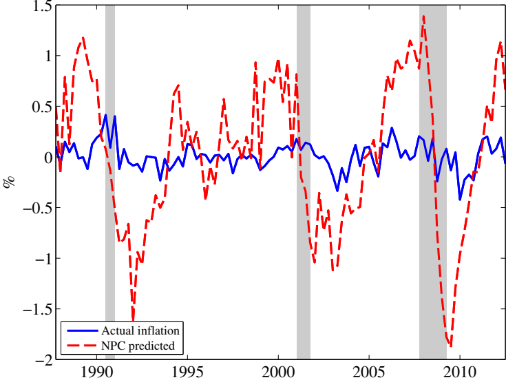
Figure C.3: Actual and predicted (by the NPC) demeaned inflation, when using HP core CPI inflation and HP hours as a measure of the output gap, using an AR(2)
